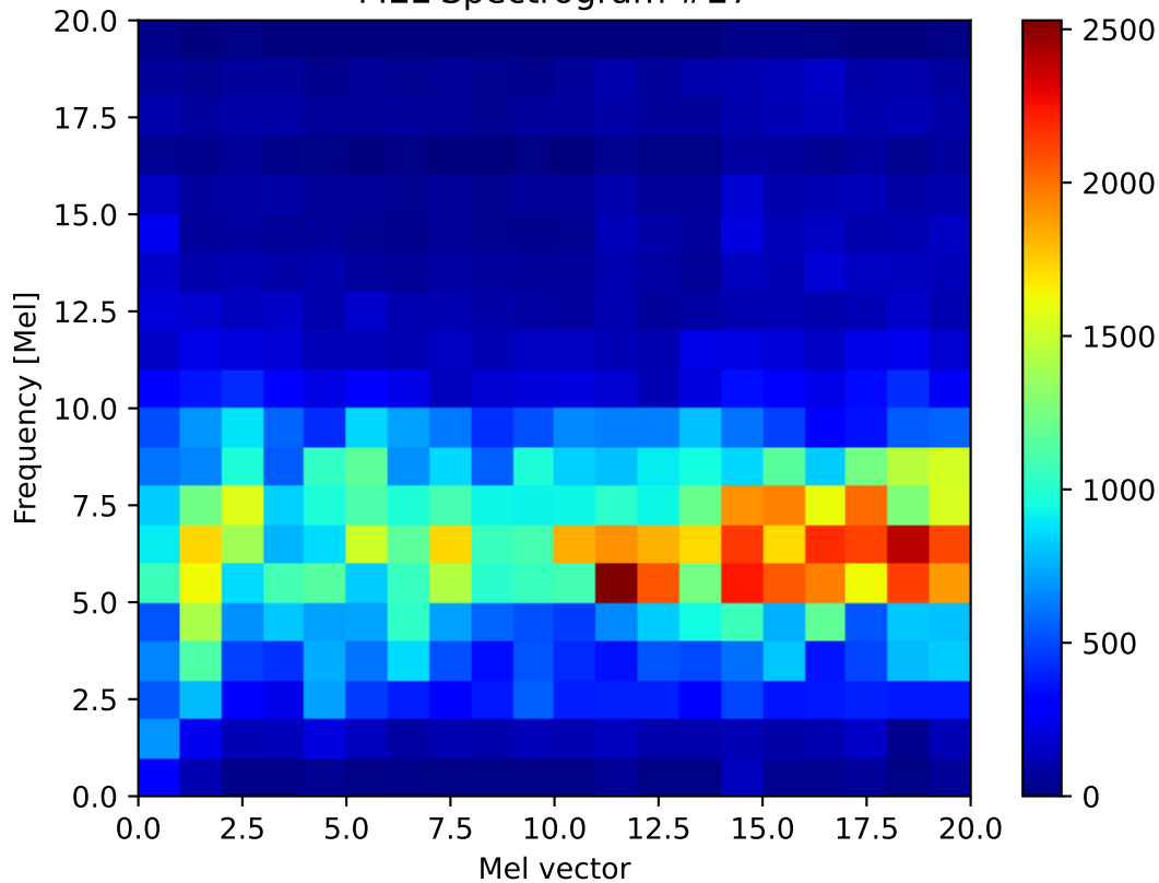
MEL Spectrogram #27
